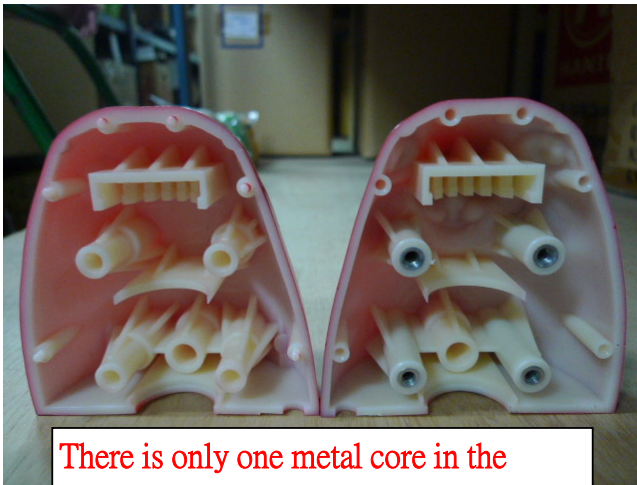
The fixed core inside the mouse head:G-UC-621-F008-EZ3 (Round 8* L80mm)
