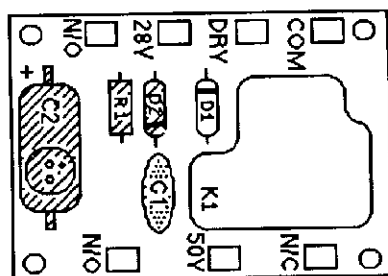
C-11677-1 Relay Snubber Board*
