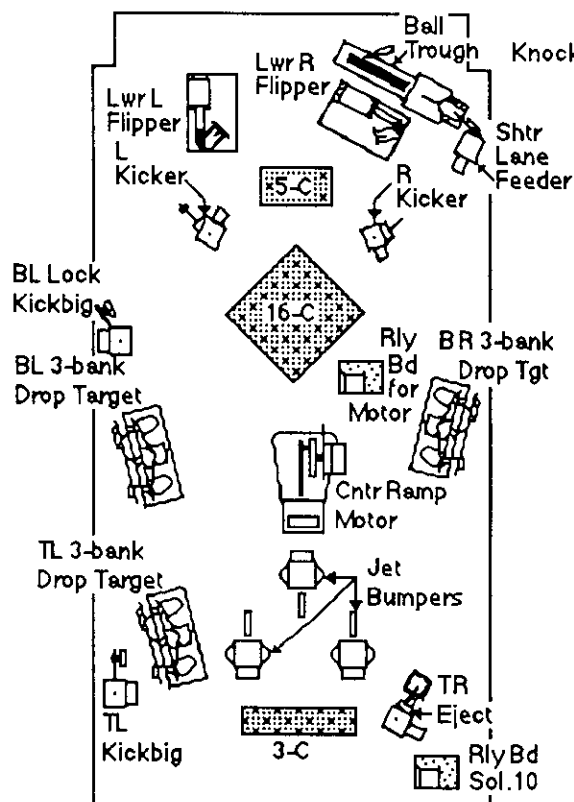
Underside of Playfield Viewed in Raised Position
