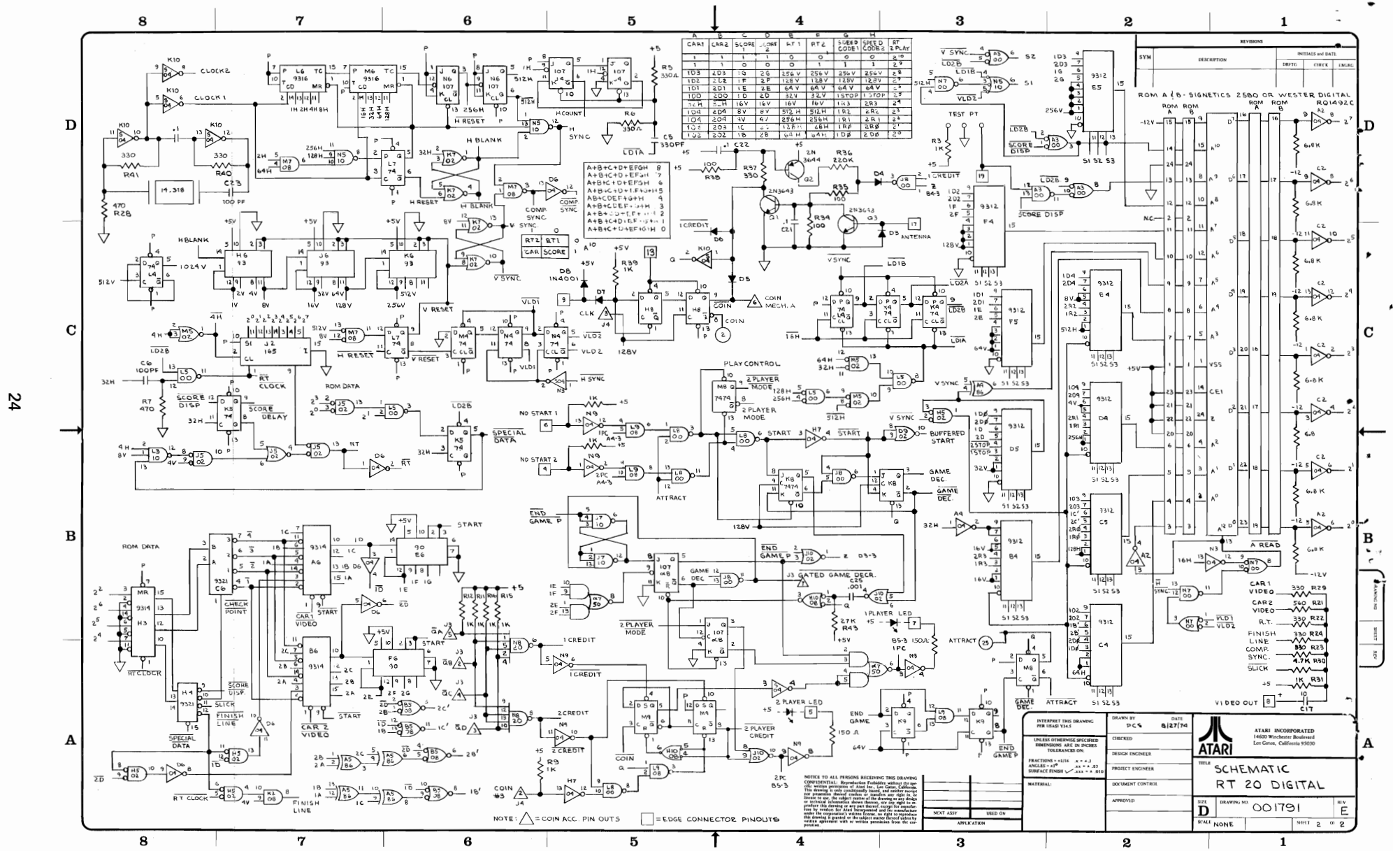
Figure 14b. Digital Board Schematic
