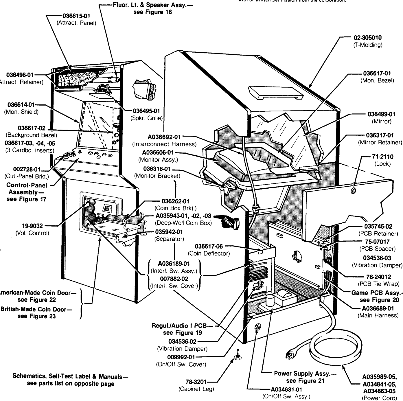
Figure 16 Cabinet-Mounted Assemblies A036500-xx B
