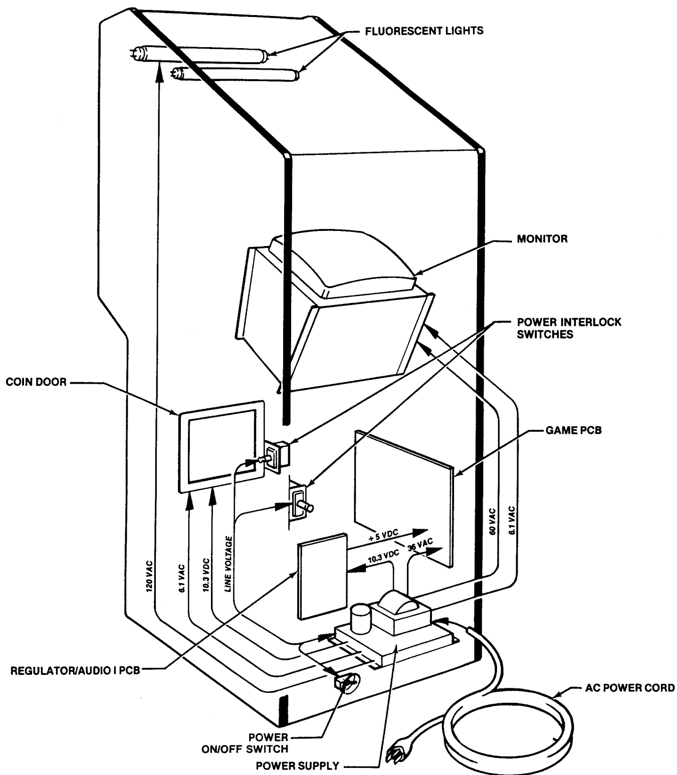
Figure 14 Power Distribution
