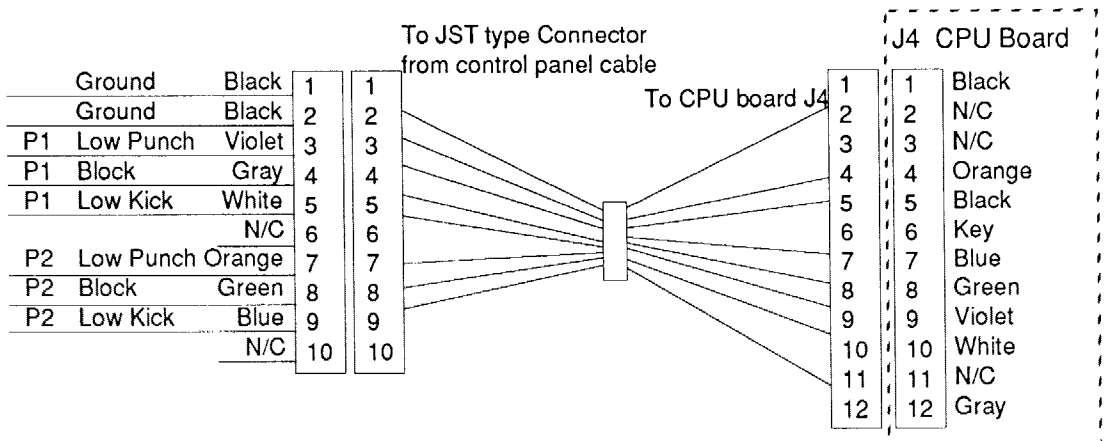
Adapter cable for STREET FIGHTER II conversion
