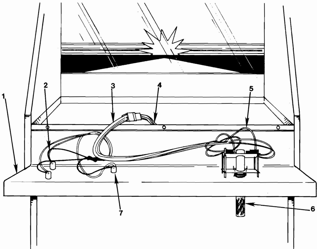
Figure 5: Control Panel (Late Production)
