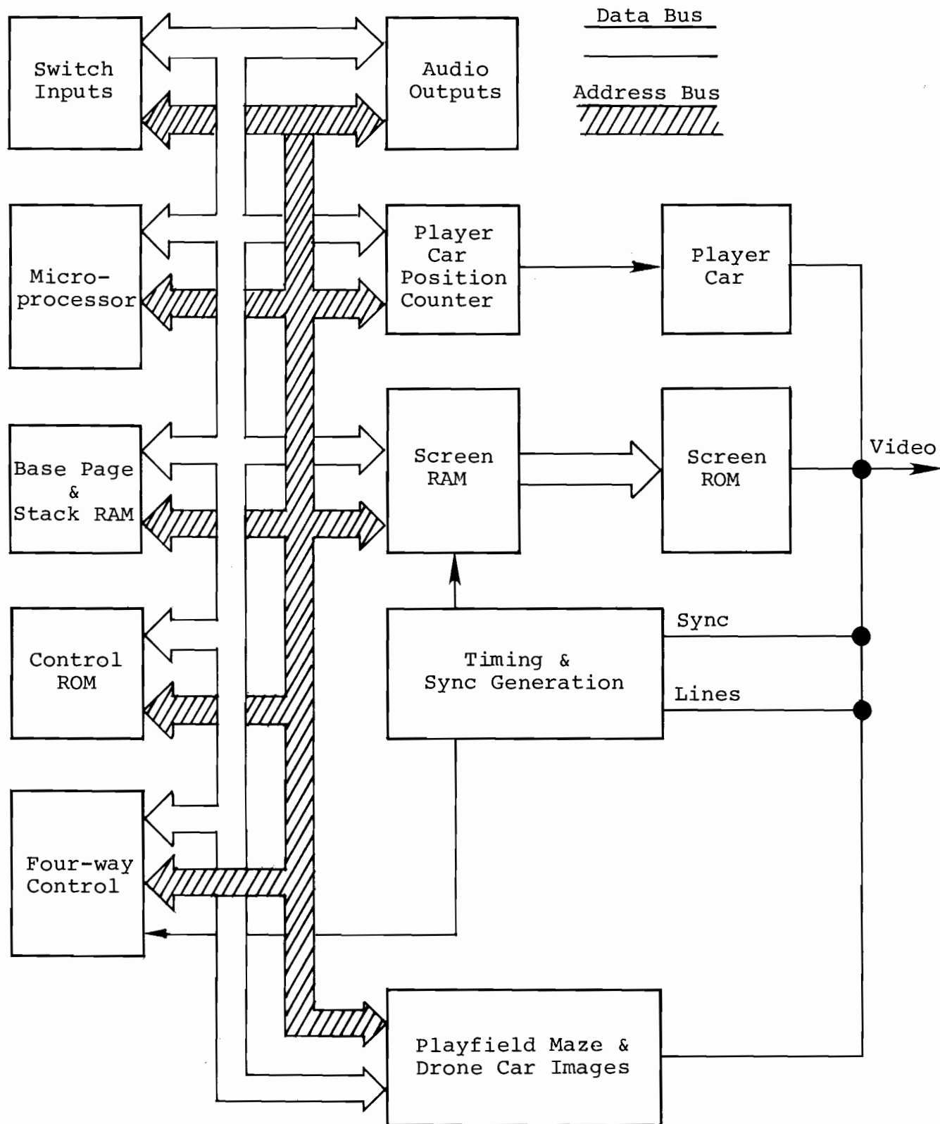
Figure 8: Logic Board Block Diagram
