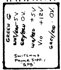
SWINDENSON SWITCHING PWR SUPPLY "SPS" MODEL 8Y6310/02
