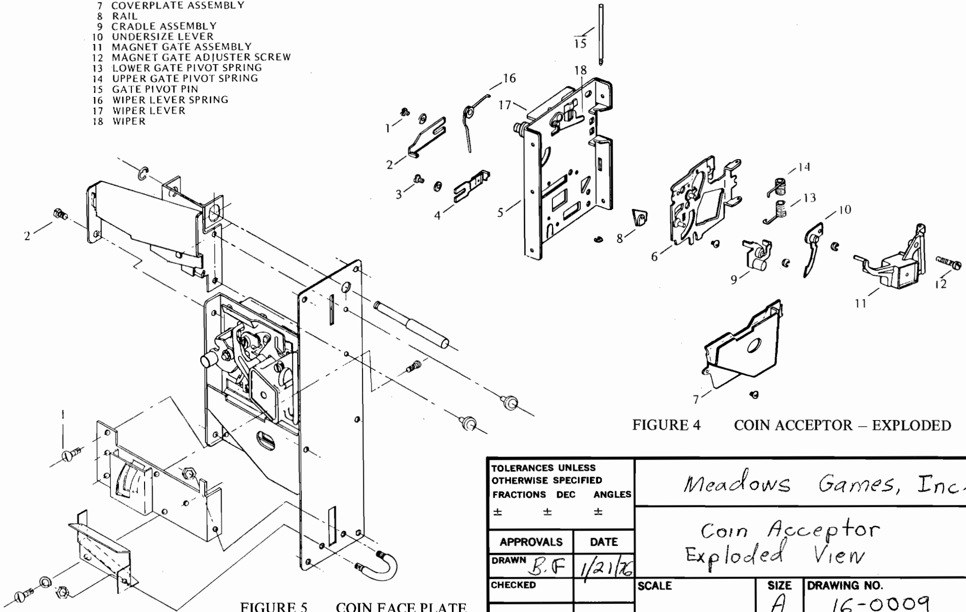
FIGURE 5 COIN FACE PLATE
