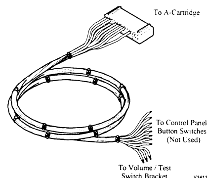
Figure 9: Auxiliary Cable Harness
