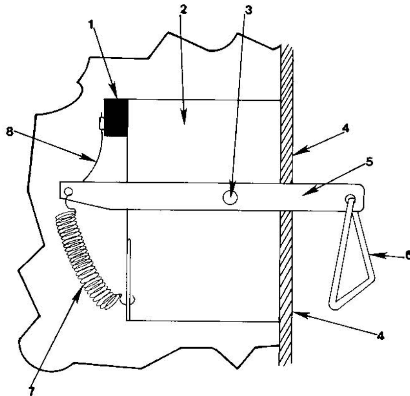
Figure 5: D-Ring Control
