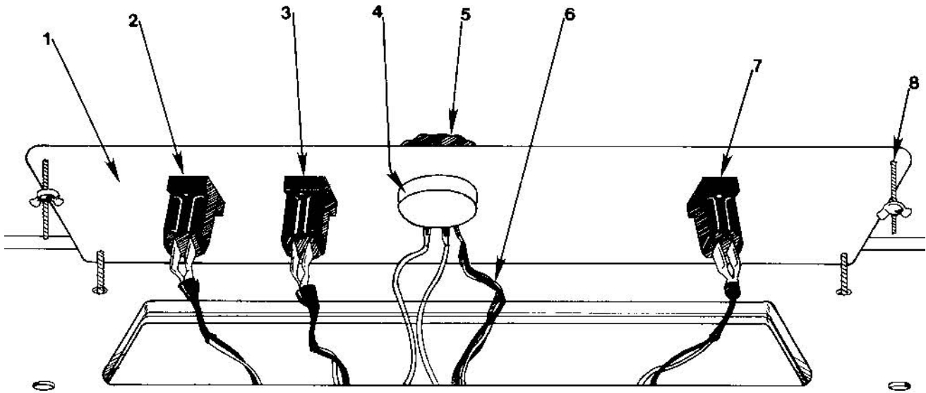
Figure 4: Control Panel
