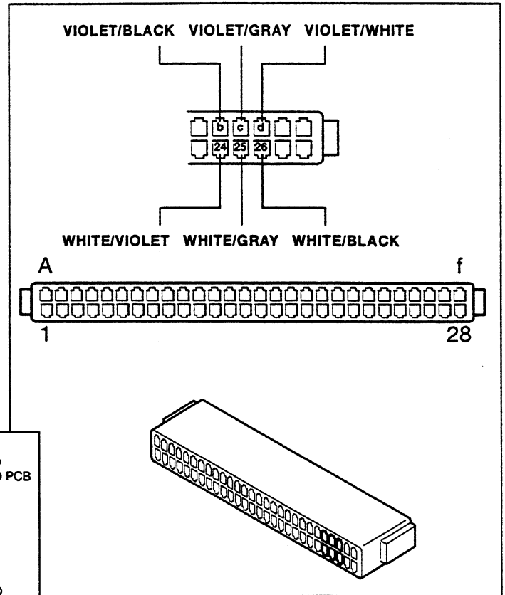
FIGURE 6 JAMMA Connector
