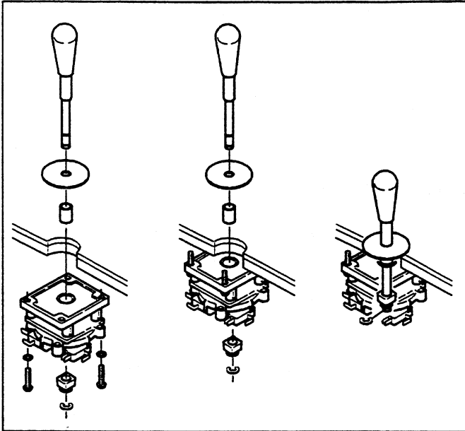
FIGURE 4 Joystick Installation
