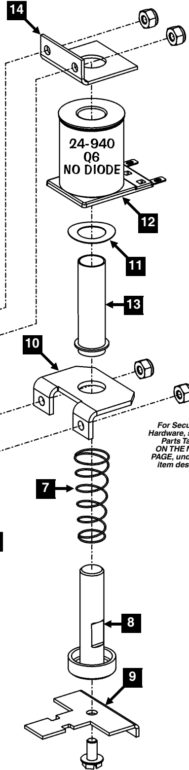
Coil Side Exploded View
