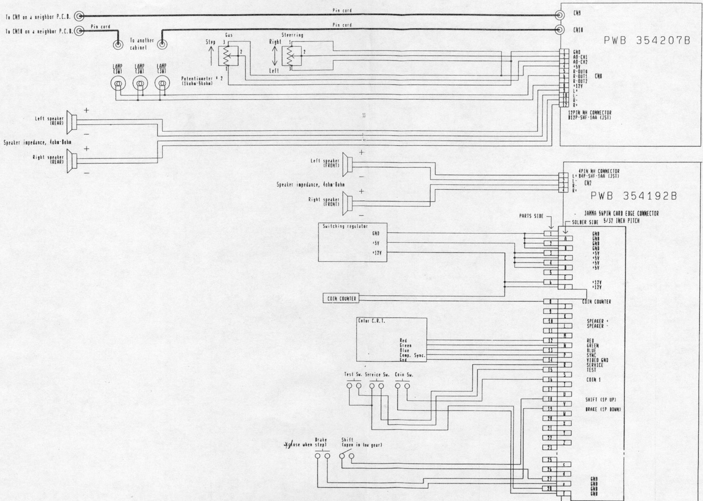
RACIN' FORCE WIRING DIAGRAM
