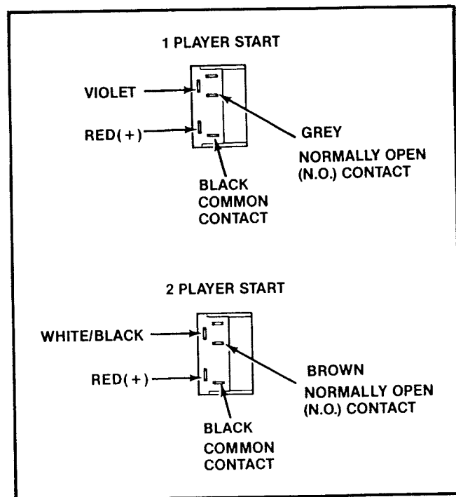
Figure 3-2 Control Panel
