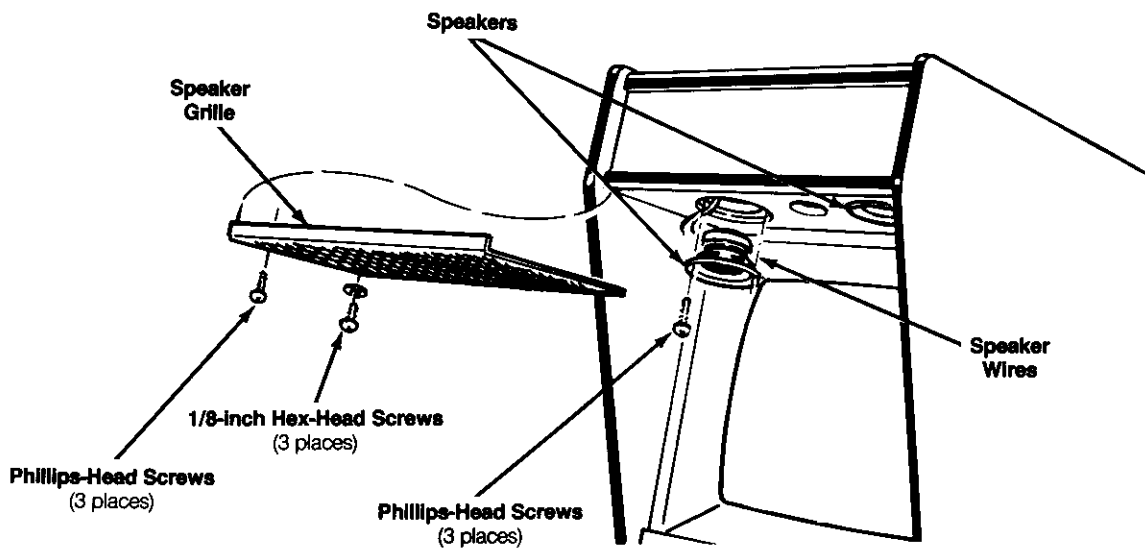
Figure 3-5 Speaker Removal
