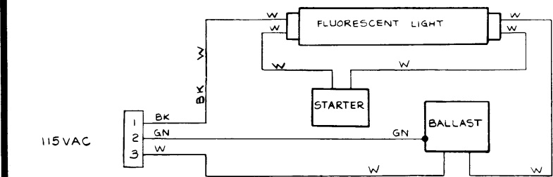
Fluorescent Light Wiring Diagram
