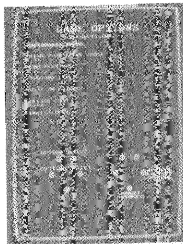
Figure 2-6 Game Options
